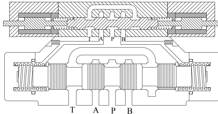
Two Stage Direction Control Valve
