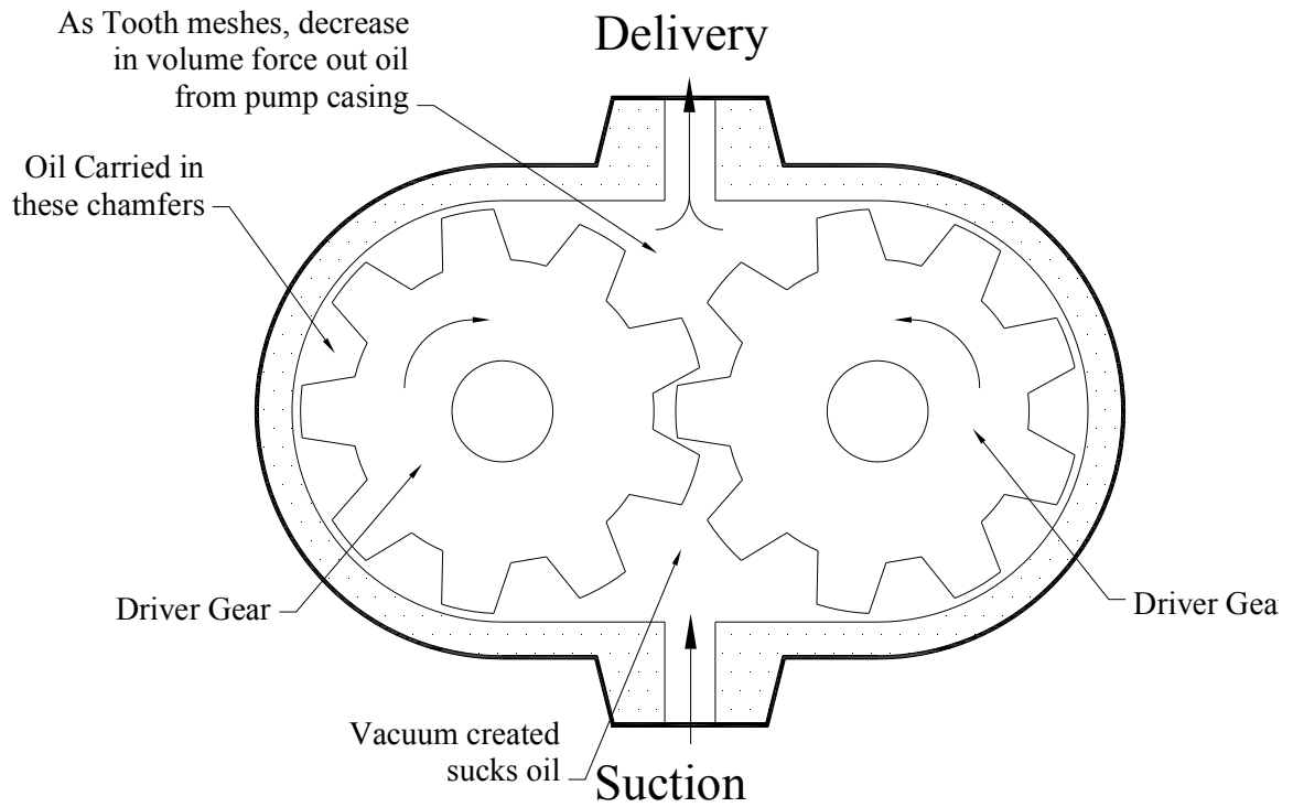
Gear Pump Figure No. 3.3
