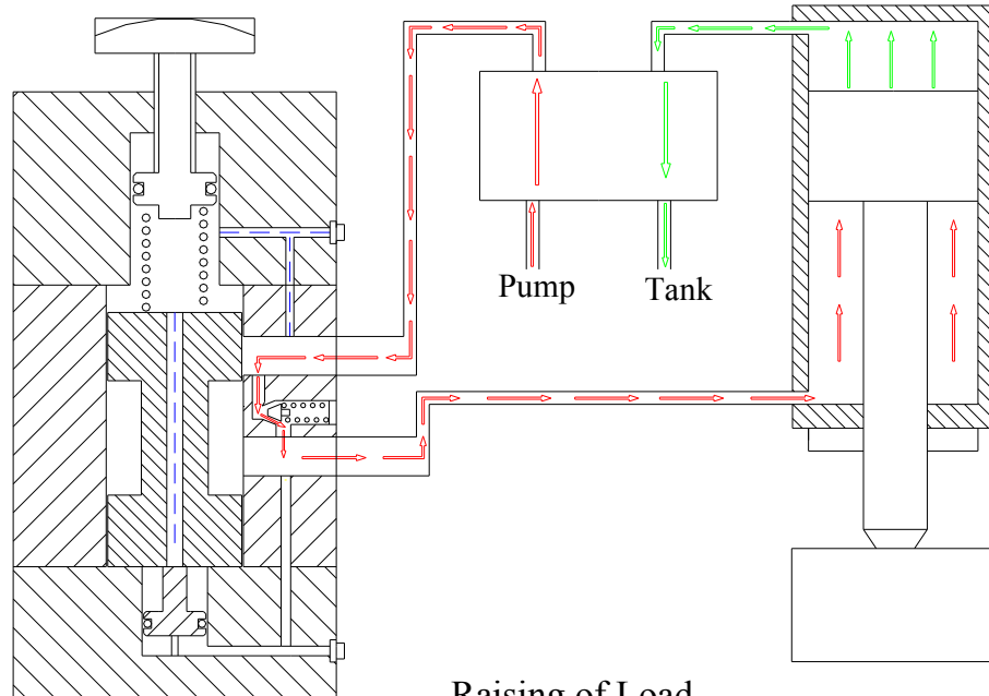
Raising of Load Figure No. 4.22
