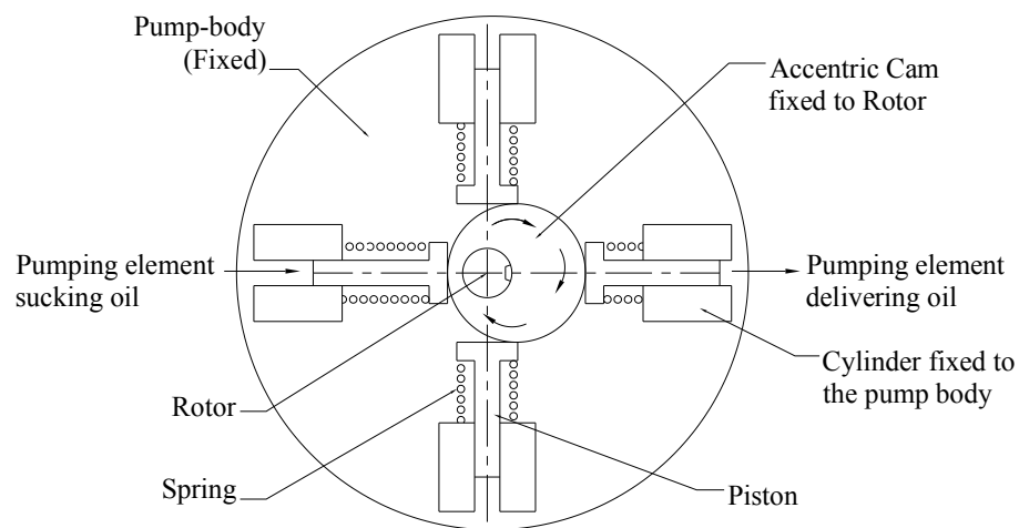
Schematic Diagram of Radial Piston Pump Figure No. 3.8
