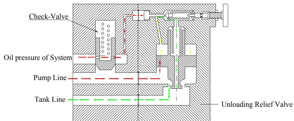
Pump getting unloaded to tank.
