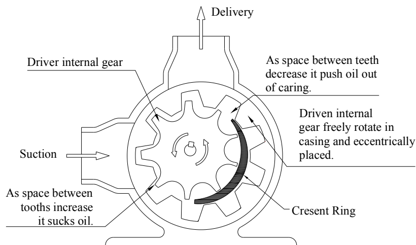
Internal Gear Pump Figure No. 3.4
