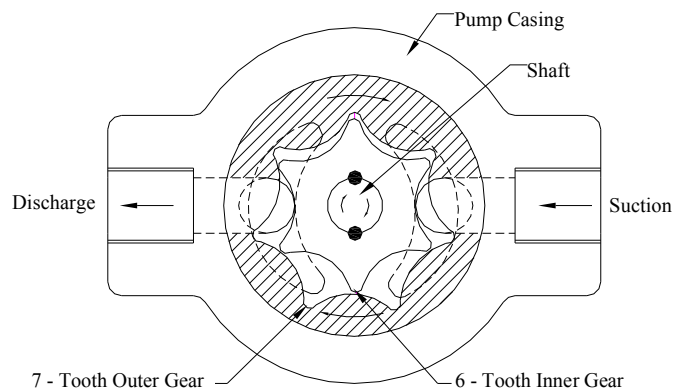
Gerotor Pump Figure No. 3.6
