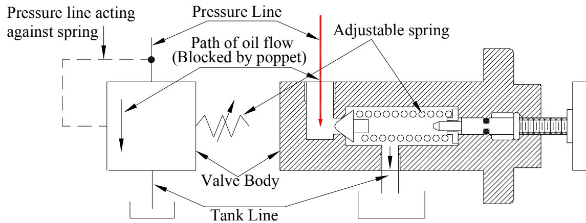
Graphic symbol for relief Valve (Cross-section)
