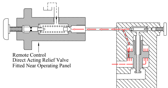
Figure No. 4.7 Pilot operated Relief Valve Fitted On Power Pack
