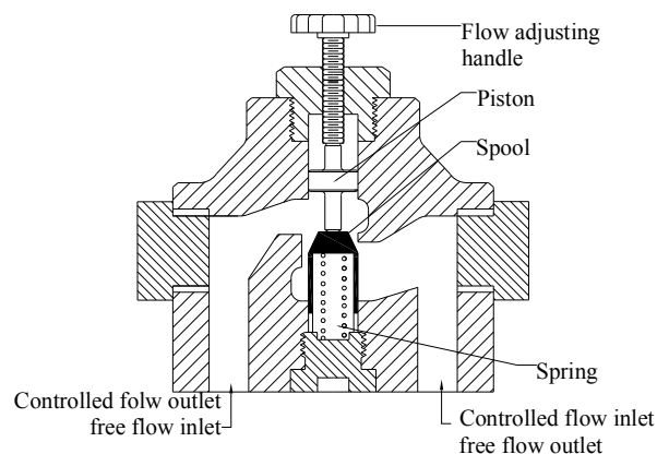
Sub-plate type construction of flow controll valve
