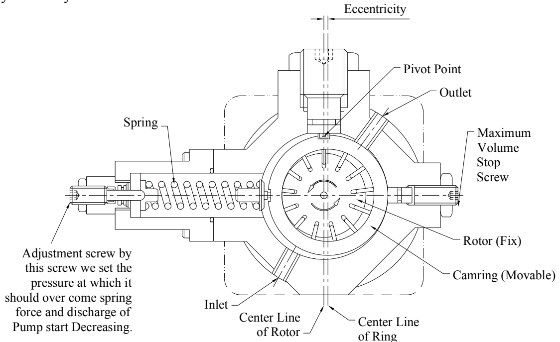
Variable Discharge Vane Pump Figure No. 3.2
