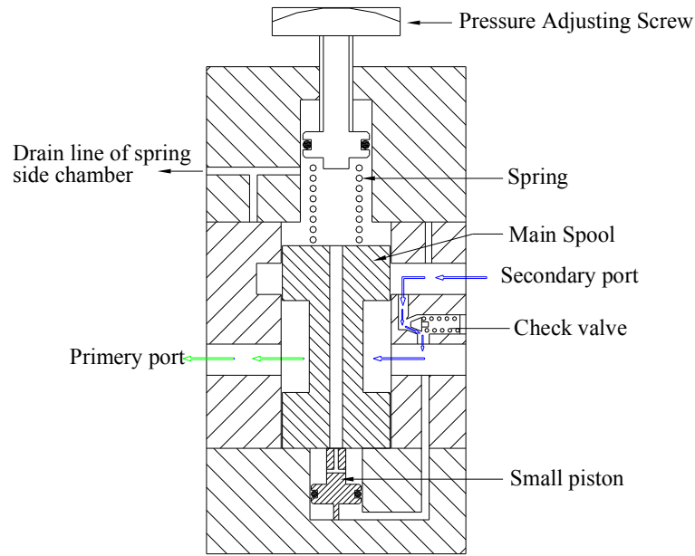
When secondary side pressure is higher than primary side in return stroke, oil by-passes through check valve
