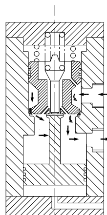
Pilot operated check valve full flow in reverse direction
