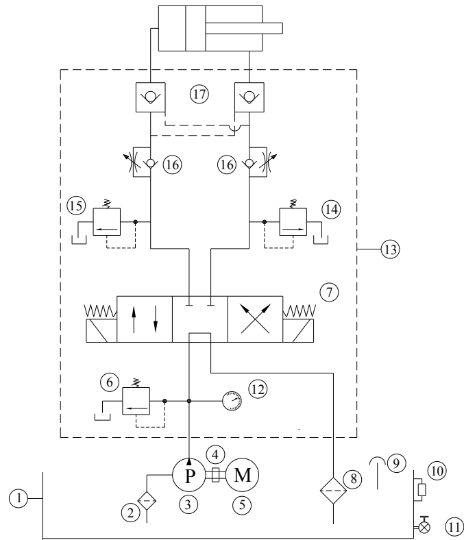
HYDRAULIC CIRCUIT DIAGRAM
