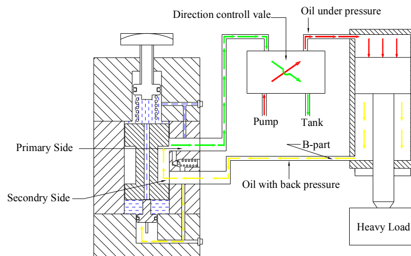
Lowering of Cylinder Figure No. 4.21
