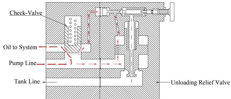
Pump supplying oil to system
