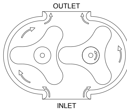
Lobe Pump Figure No. 3.5
