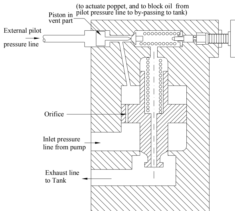
Unloading Relief Valve
